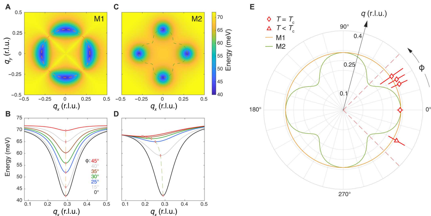
Fig. 3. Models of phonon softening for QDCs and directional order. (A and C) Phonon dispersion for M1 and M2, as described in the text. (B and D) Momentum q cuts of the phonon dispersion at different \phi for the simulated data in (A) and (C), respectively. The dashed orange and green lines in (A) to (D) identify the location of the phonon softening in the q_x - q_y plane. (E) Polar plot contrasting M1 and M2 models (orange and green solid lines) and the experimental data (red symbols). The error bars in (E) are obtained from the fits to the phonon dispersion in Fig. 2B. See Materials and Methods for more details. r.l.u., reciprocal lattice units.
