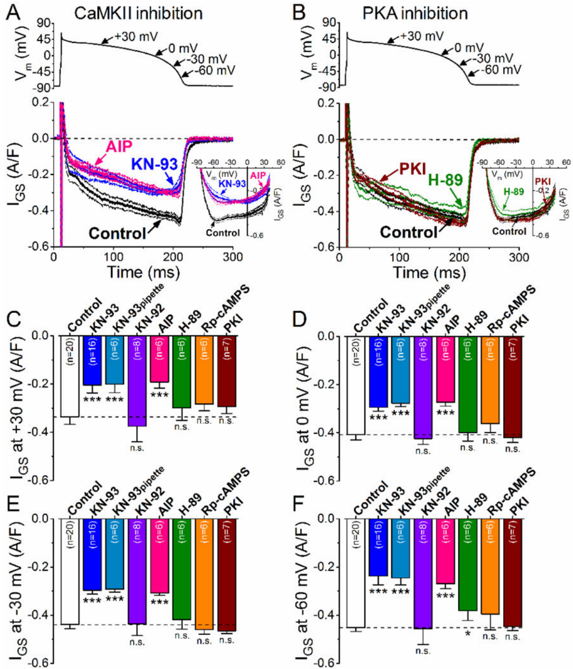
Figure 3. CaMKII-dependent and PKA-dependent regulation of basal I_{NaL} under AP-clamp. (A) GS-458967-sensitive current ( I_{GS} ) traces (mean±SEM) under AP-clamp in control and after CaMKII inhibition using KN-93 (1 pM) or AIP (1 \mu M). The physiological intracellular Ca^{2+} cycling was preserved, and 2 Hz steady-state pacing was applied. I-V trajectories of I_{GS} under AP-clamp are shown in inset. (B) I_{GS} traces (mean±SEM) under AP-clamp in control and after PKA inhibition using H-89 (1 \mu M) or PKI (1 \mu M). I-V relationships are shown in the inset. (C-E) I_{GS} density at different voltages during AP repolarization. CaMKII inhibition with KN-93 or AIP significantly decreased I_{NaL} at all voltages, whereas KN-92 (1
