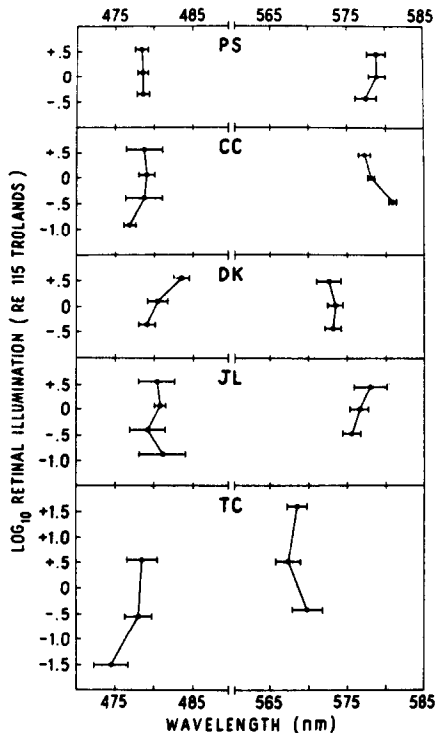
Fig. 4. Mean value of equilibrium blue (left) and equilibrium yellow (right) spectral loci, at various luminance levels, for five observers. Note the break in the wavelength abscissa between 485 and 565 nm. Error bars are 80 per cent confidence intervals based on between-session variability.
