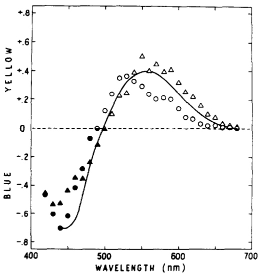
Fig. 2. Yellow/blue cancellation coefficient (details as in Fig. 1).
