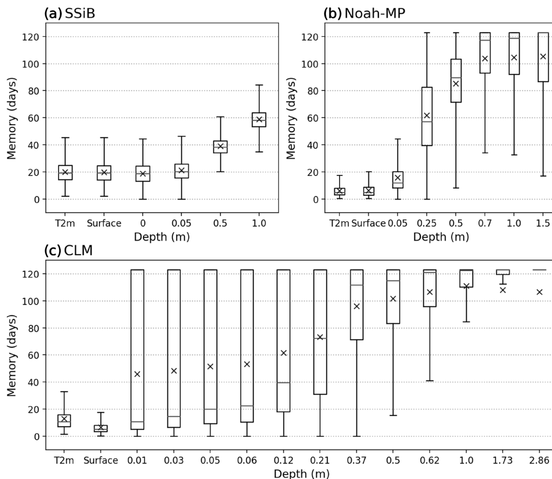
Fig. 5 Boxplots of T2m/surface/soil memories (units: days) over Tibetan Plateau in the +5 °C experiments with different land models, in which the digital along the x-axis are the depths of the soil layers. In addition, the markers “x” indicate the means and the upper (lower)
