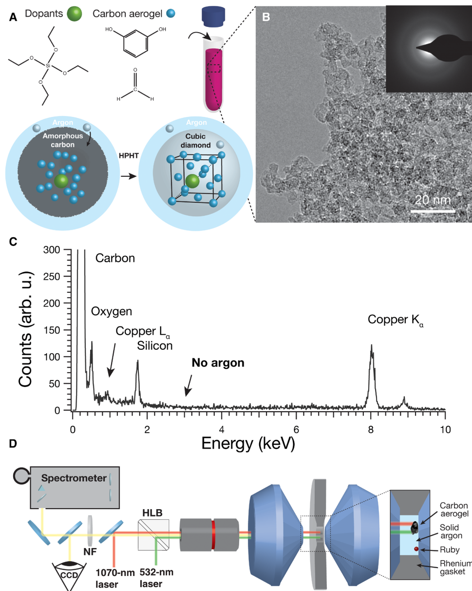
Fig. 1. Carbon precursor doping mechanism and characterization. (A) Schematic representing the synthesis and doping of carbon aerogels, including BF-TEM image with SAED inset. To incorporate them within the carbon aerogel grains, we introduce dopants simultaneously with resorcinol and formaldehyde. Upon conversion to diamond at high pressure and high temperature, dopants remain inside the diamond lattice as color centers. (B) A TEM image with SAED of the doped carbon aerogel illustrates the carbon precursor morphology and lack of crystallinity. (C) EDS spectra of the carbon aerogel as synthesized only show the presence of carbon, silicon, and oxygen. Copper signal comes from the TEM grid. arb. u., arbitrary units. (D) Schematic showing a 1070-nm heating laser or polarized 532-nm Raman and photoluminescence (PL) laser focused into the pressurized DAC, which is loaded with a carbon aerogel precursor, ruby for pressure measurements, and solid argon pressure media, contained by a rhenium gasket. CCD, charge-coupled device; NF, notch filter; HLB, holographic beamsplitter cube.
