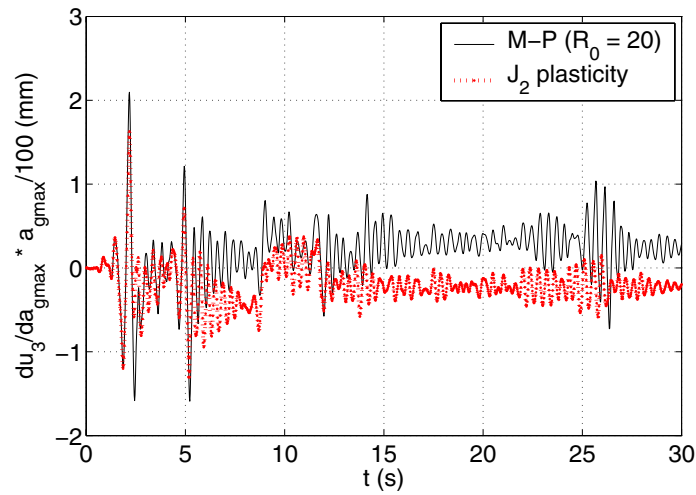
Figure 9. Normalized sensitivity of roof displacement u_3 to peak ground acceleration a_{g,max} (dynamic analysis).
