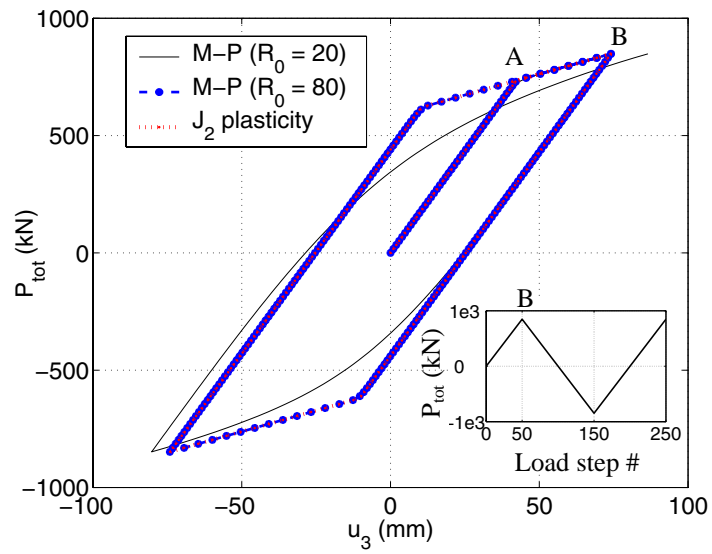
Figure 3. Total base shear, P_{tot} , versus roof displacement, u_3 , for quasi-static cyclic loading and different constitutive models.
