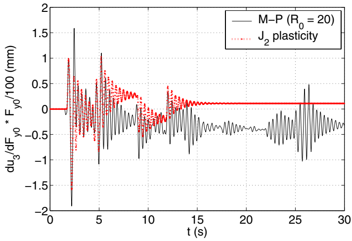
Figure 8. Normalized sensitivity of roof displacement u_3 to initial yield force F_{y0} (dynamic analysis).
