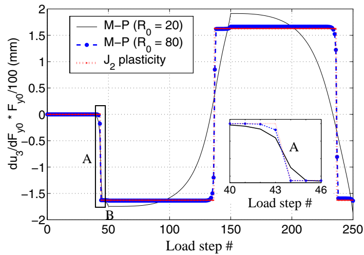
Figure 4. Normalized sensitivity of roof displacement u_3 to initial yield force F_{y0} (quasi-static cyclic loading).
