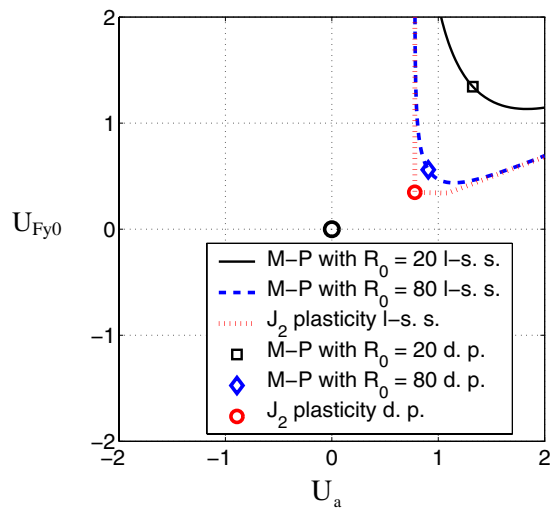
Figure 21. Limit-state surfaces (l-s. s.) and design points (d. p.) for u_{lim} = -33mm at time t = 1.66s (dynamic analysis).
