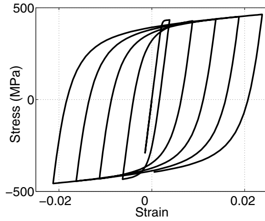
Figure 1. Cyclic stress-strain response behavior of structural steel modeled using Menegotto-Pinto model.
