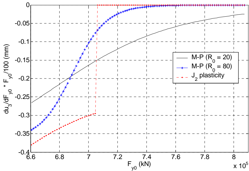
Figure 10. Normalized sensitivity of roof displacement u_3 to initial yield force F_{y0} at time t = 1.66s with fixed peak ground acceleration a_{g,max} .
