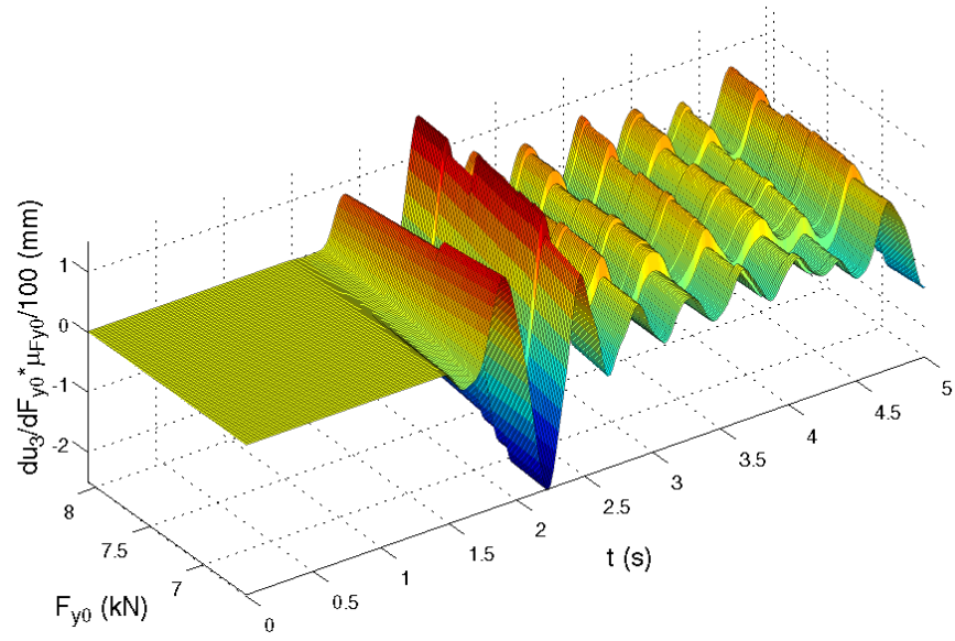
Figure 15. Time histories (for 0 \leq t \leq 5s ) of normalized sensitivities of the displacement u_3 to initial yield force F_{y0} for fixed peak ground acceleration a_{g,max} and variable initial yield force F_{y0} : dynamic analysis using the M-P ( R_0 = 20 ) model and \Delta t = 0.02s .
