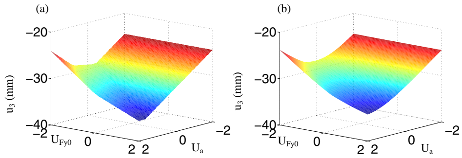
Figure 20. Response surfaces at time t = 1.66s for dynamic analysis of example structure modeled with: (a) J_2 plasticity model, and (b) M-P ( R_0 = 20 ) model.
