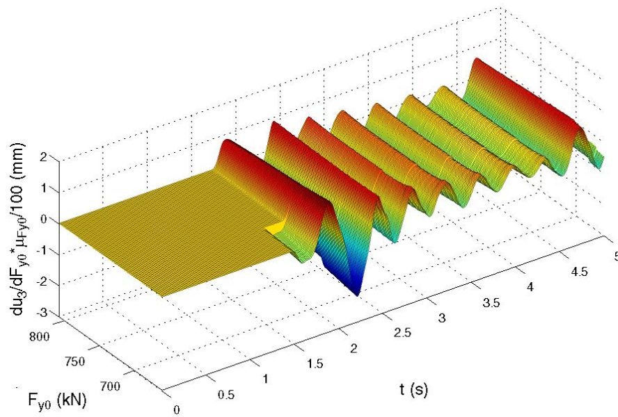
Figure 14. Time histories (for 0 \leq t \leq 5s ) of normalized sensitivities of the displacement u_3 to initial yield force F_{y0} for fixed peak ground acceleration a_{g,max} and variable initial yield force F_{y0} : dynamic analysis using the J_2 plasticity model and \Delta t = 0.001s .
