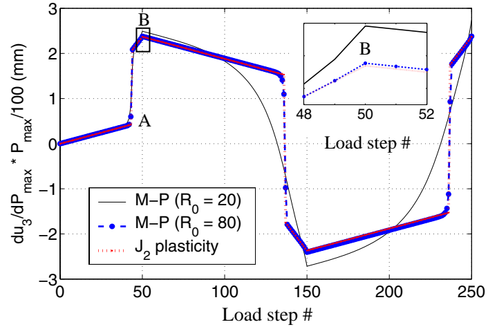
Figure 5. Normalized sensitivity of roof displacement u_3 to loading parameter P_{max} (quasi-static cyclic loading).
