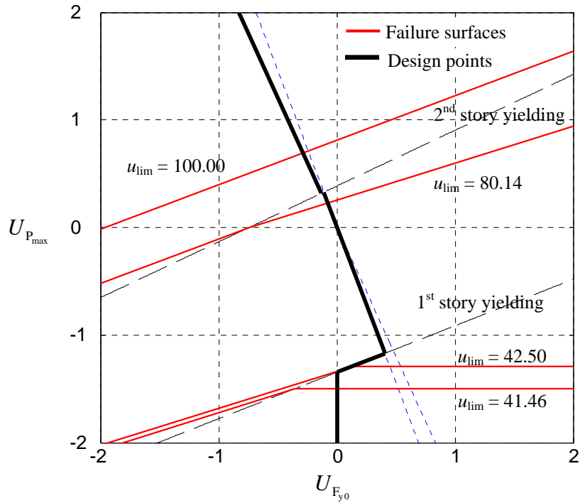
Figure 17. Locus of the design points for varying u_{lim} , when the example structure is modeled using the J_2 plasticity model (probabilistic pushover analysis).
