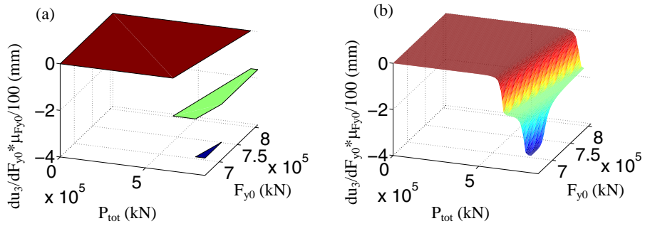
Figure 18. Normalized sensitivities of roof displacement u_3 to initial yield force F_{y0} for varying F_{y0} : (a) J_2 plasticity model, and (b) M-P ( R_0 = 20 ) model.
