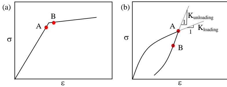
Figure 6. Examples of branches of material constitutive models: (a) loading branch with elastic-to-plastic material state transition (discontinuous response sensitivities), and (b) smooth loading and unloading branches at unloading event (continuous response sensitivities).
