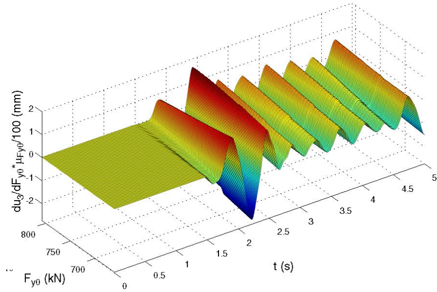
Figure 13. Time histories (for 0 \leq t \leq 5s ) of normalized sensitivities of the displacement u_3 to initial yield force F_{y0} for fixed peak ground acceleration a_{g,max} and variable initial yield force F_{y0} : dynamic analysis using the M-P ( R_0 = 20 ) model and \Delta t = 0.001s .
