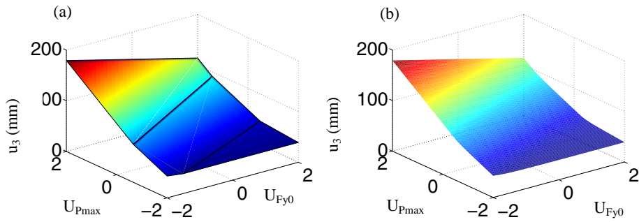
Figure 16. Response surfaces for quasi-static pushover analysis of example structure modeled using: (a) J_2 plasticity model, and (b) M-P ( R_0 = 20 ) model.
