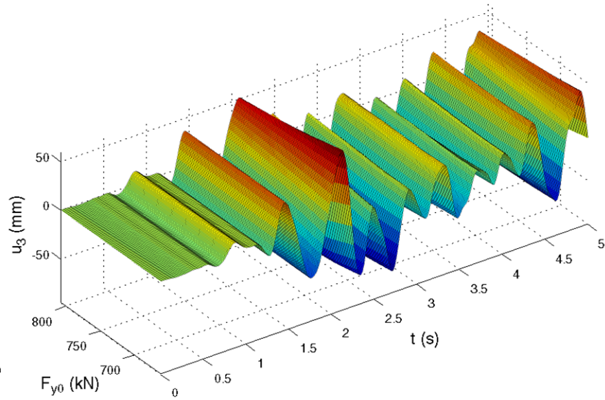
Figure 11. Time histories (for 0 \leq t \leq 5s ) of displacement u_3 for fixed peak ground acceleration a_{g,max} and variable initial yield force F_{y0} : dynamic analysis using the M-P ( R_0 = 20 ) model and \Delta t = 0.001s .
