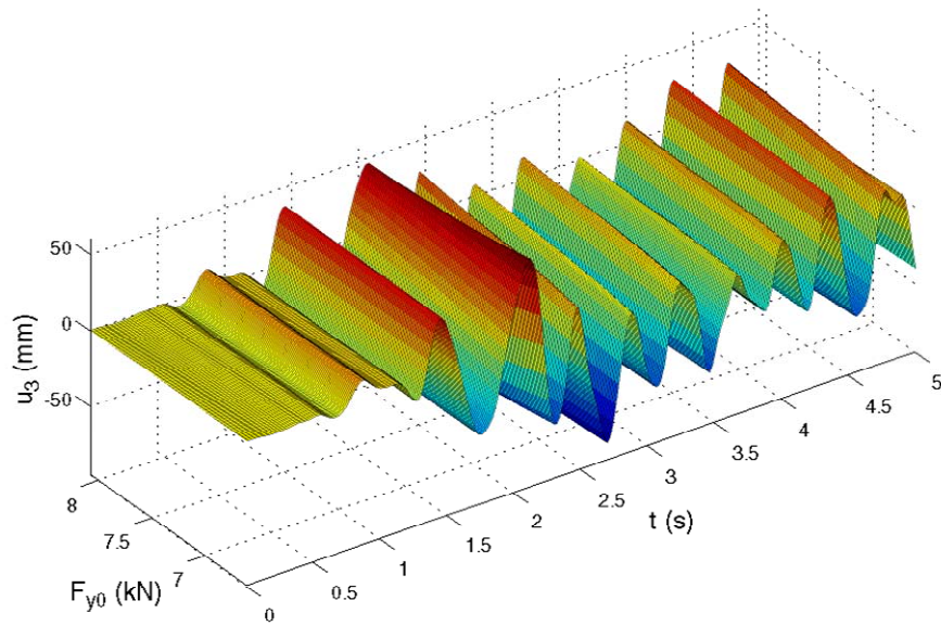
Figure 12. Time histories (for 0 \leq t \leq 5s ) of displacement u_3 for fixed peak ground acceleration a_{g,max} and variable initial yield force F_{y0} : dynamic analysis using the J_2 plasticity model and \Delta t = 0.001s .
