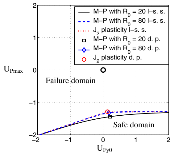
Figure 19. Limit-state surfaces (l-s. s.) and design points (d. p.) for u_{lim} = 42.5\text{mm} (probabilistic pushover analysis).
