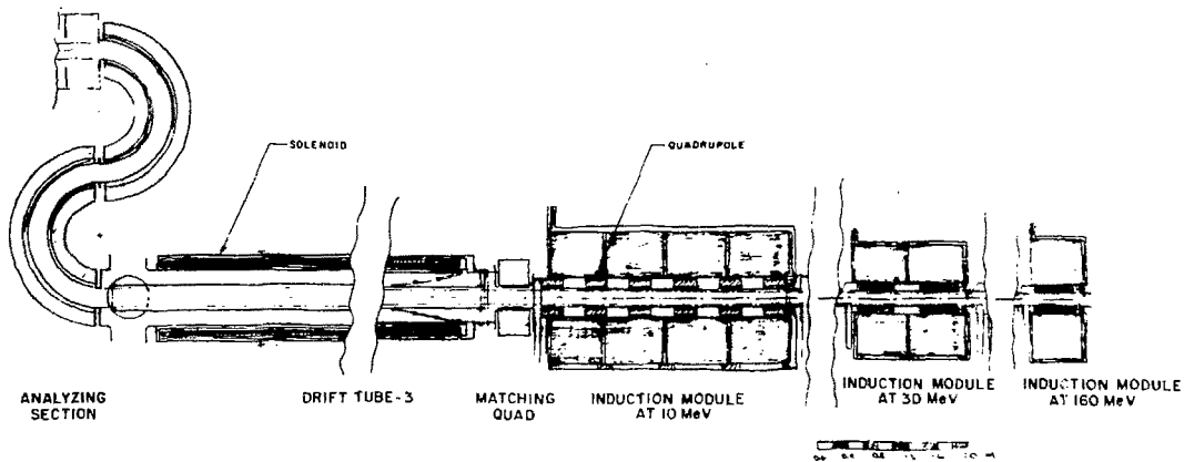
160 MeV, A 4+ (A > 200) INJECTOR FOR IMJ, 156TW, 155 \mu C
