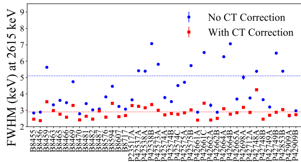
FIG. 6. Energy resolution (FWHM, statistics only) at 2615 keV for all operating detectors in DS6a before (blue points) and after (red points) the charge trapping correction. The x -axis is the detector ID. Detector IDs beginning with “B” and “P” are natural and enriched Ge detectors, respectively. The average resolution after the charge trapping correction (red line) represents a \approx 30\% improvement. The variation between detectors is mostly due to differing crystal impurities and maximum drift times. Figure from Ref. [26].
