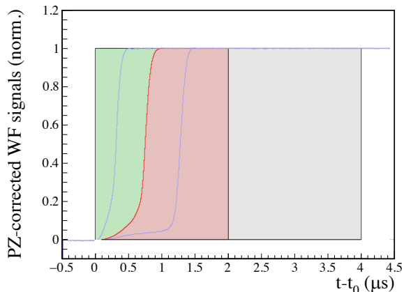
FIG. 13. Visualization of the alternative charge trapping correction. The value of D is represented by the area shaded green, given by the difference between the 2\text{-}\mu s integrated waveform regions represented by gray and red. For reference, pulses with shorter and longer drift times are included; these would have smaller and larger values of D , respectively.
