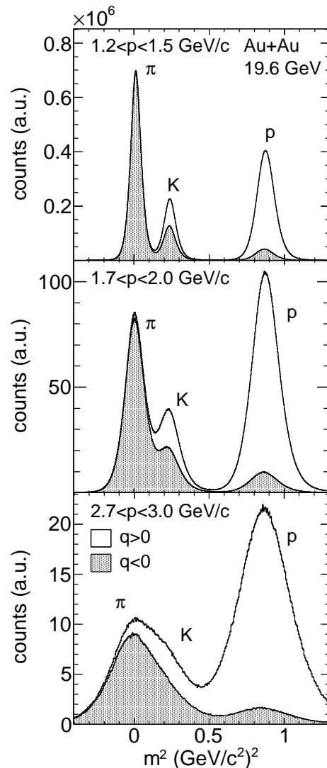
FIG. 3. The mass-squared, m^2 , distributions for reconstructed positive ( q>0 ) and negative ( q<0 ) charged particles from 0–80% central Au+Au collisions at the beam energy of 19.6 GeV. Three different momentum ranges are shown.
