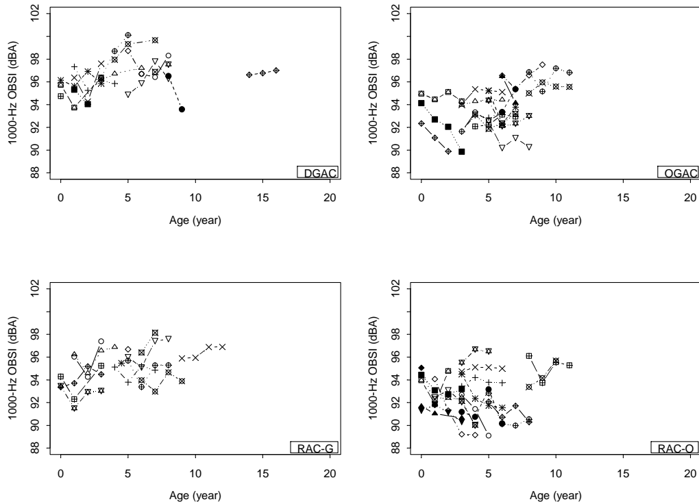
Figure A.20: Sound intensity at 1,000 Hz over four years for each pavement section.
