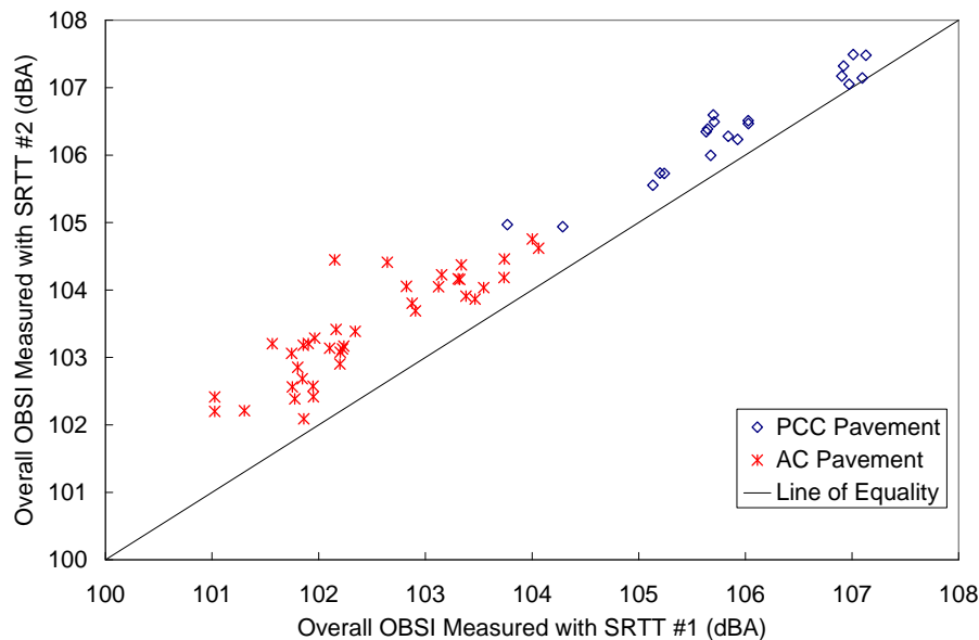
Figure 5.1: Comparison of overall OBSI values measured with SRTT #1 and SRTT #2.
