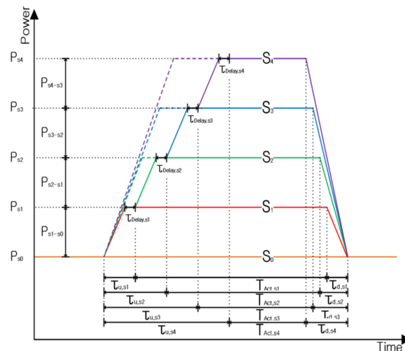
Figure 8. Modeling of node wake-up signal processing.
