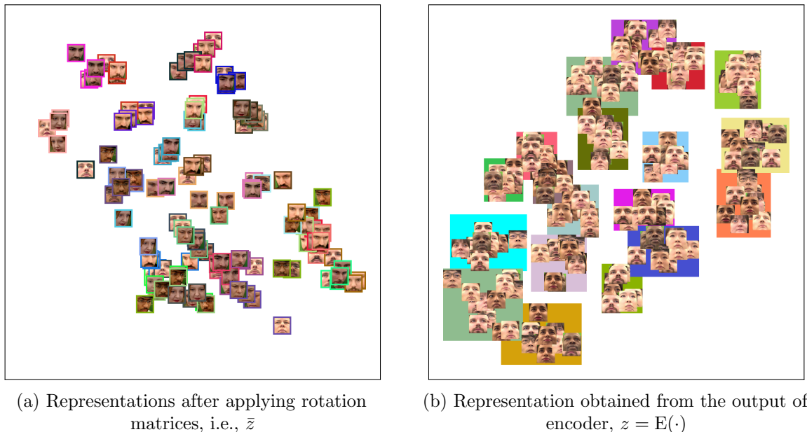
Figure 5: t-SNE visualization. Qualitative visualization of gaze representations in 2-dimensional space using the t-SNE algorithm. (a) shows the visualization of projection embeddings for multi-view images obtained after applying rotation matrices, i.e., \bar{z} . The images with the same timestamp for all four views are highlighted using the same border color. (b) depicts representations for the output of encoder network, i.e., z = E(\cdot) obtained for images from single camera viewpoint. Best viewed in color and after zooming.
