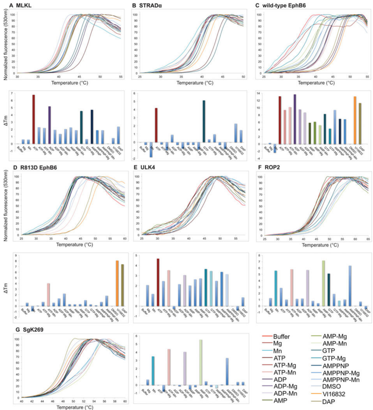
Figure 3. Thermal denaturation curves and T_m analyses of Class 2 (nucleotide binding) and Class 3 (cation binding) pseudokinases
