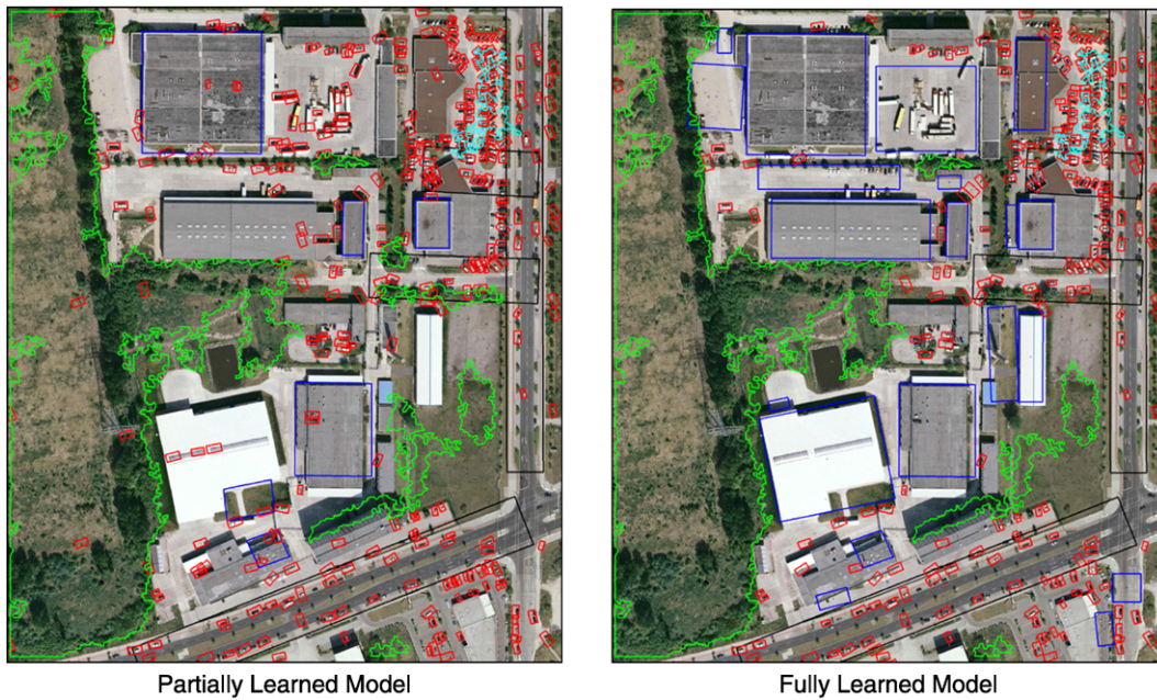
Fig. 25 A comparison of inference results for the model learned with a very high \epsilon_1 versus a rather low \epsilon_1 (i.e. fewer relationships are added to the first model). The partially learned model is missing a lot of over-
