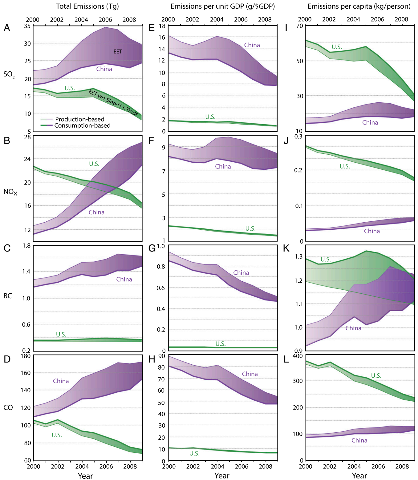
Fig. 1. Air pollutants embodied in Chinese trade between 2000 and 2009. (A–D) Production-based emissions (thin lines), consumption-based emissions (thick lines), and their differences (i.e., Chinese EET associated with its trade with the rest of the world in purple shading, and EET associated with Sino-US trade alone in green shading). All Chinese emissions are calculated here, the US production-based emissions are taken from the National Emissions Inventory, and the US consumption-based emissions are derived based on production-based emissions and Sino-US trade-related emissions. Although China’s production-based emissions are growing rapidly, its EET are equivalent to substantial fractions of the production-based emissions. Similarly, the EET due to Sino-US trade are equivalent to large proportions of the production-based US emissions since 2006. (E–H) Emissions per unit GDP. Although China’s production-based emissions per unit GDP have been decreasing, its consumption-based emissions per unit GDP have decreased less significantly or have increased since 2008. (I–L) Emissions per capita. Per capita emissions are very different between the United States and China, and this disparity is increased when the consumption-based emissions are considered. For data sources, see SI Appendix, Table S1, footnote .
