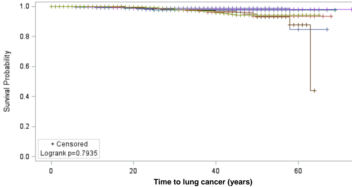
Kaplan Meier survival curve for length of time (after initial employment in the shipyard) until occurrence of lung cancer stratified by asbestos exposure and duration of employment
