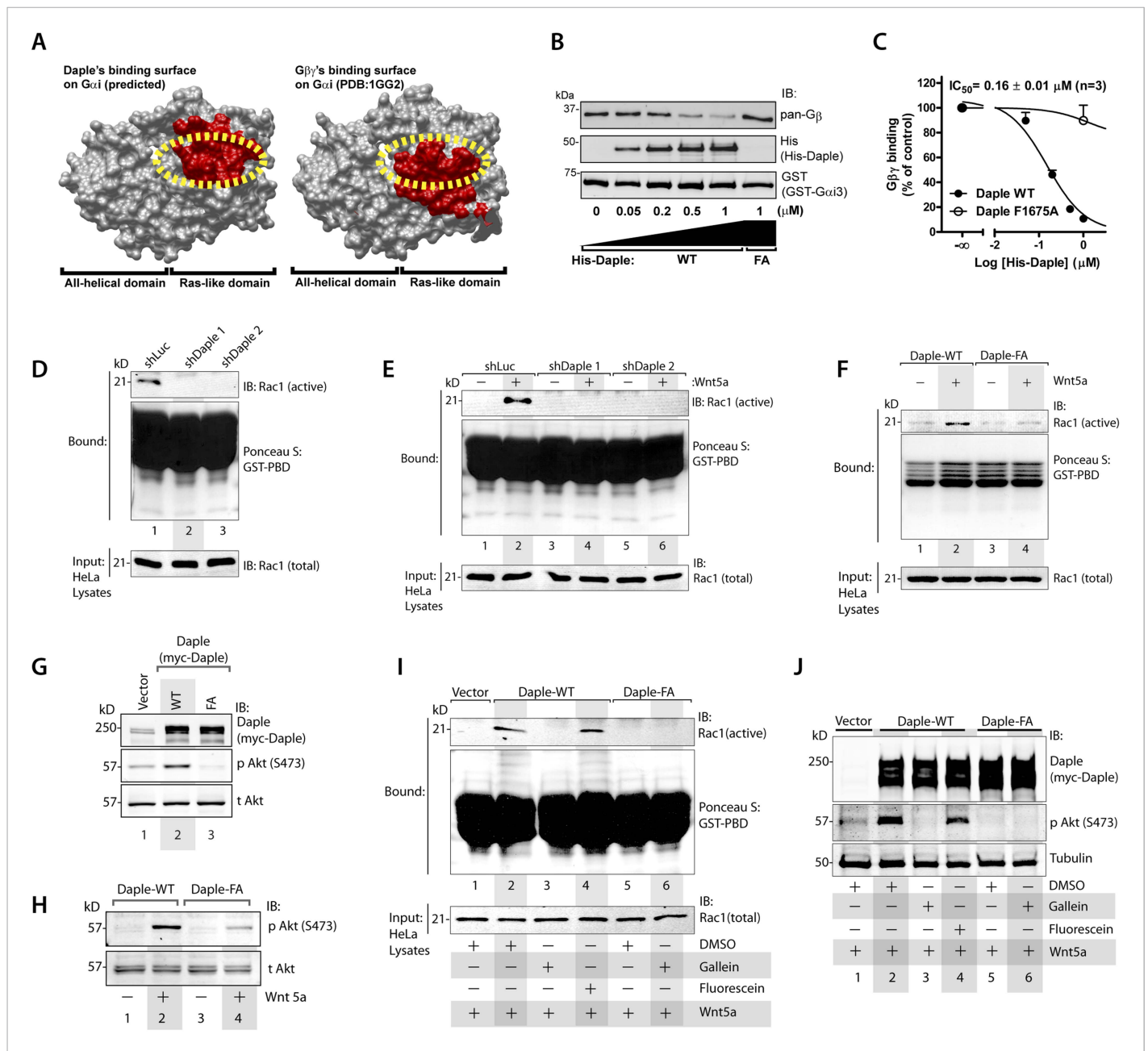
Figure 3. Daple's GBA motif triggers the release of 'free' Gβγ subunits, which in turn enhance Rac1 and PI3K-Akt signaling. (A) Daple's GBA motif and Gβγ subunits are predicted to dock onto an overlapping binding site on Gαi. Binding areas (in red) for Daple (left) or Gβγ (right) on Gαi (solid gray) were extracted from a homology-based model of Daple-Gαi3 and the crystal structure of the Gαi1-Gβγ complex (Protein Data Bank [PDB]: 1GG2), respectively. (B, C) Daple displaces Gβγ subunits from Gαi3 via its GBA motif. GST-Gαi3-Gβγ preformed complexes immobilized on glutathione beads were incubated with increasing concentrations of His-Daple-CT WT or F1675A (FA). Bound proteins were analyzed by IB (B) and Gβγ binding data fitted to a single-site competition curve (C) . Mean ± S.E.M. of three independent experiments. (D, E) Activation of Rac1 is impaired in Daple-depleted HeLa cells. Control (shLuc) or two clones of Daple-depleted HeLa cell lines (sh Daple 1 and 2) (described in Figure 2—figure supplement 1A,B ) were incubated in 2% serum media (D) or starved and treated (+) or not (–) with Wnt5a (0.1 mg/ml) for 5 min (E) and analyzed for Rac1 activation by pull-down assays using GST-PBD. (F) Activation of Rac1 is impaired in cells expressing Daple-F1675A (FA) mutant compared to those expressing Daple-WT. Daple-depleted (sh Daple 1) HeLa cells transiently transfected with myc-Daple-WT or FA were starved and stimulated with Wnt5a and analyzed for Rac1 activation as in E . (G, H) Daple's GBA motif is required for activation of PI3K-Akt signaling in HeLa cells, as determined by phosphorylation of Akt at S473. Daple-depleted (sh Daple 1) HeLa cells transiently transfected with myc-Daple WT or F1675A (FA) were incubated in a 2% serum media (G) or in a 0.2% serum media overnight and treated (+) or not (–) with 0.1 mg/ml Wnt5a for 5 min (H) prior to lysis. Equal aliquots of whole-cell lysates were analyzed for Akt phosphorylation (pAkt S473) by IB. (I, J) Inhibition of Gβγ signaling impairs Daple-dependent activation of Rac1 and Akt. Daple-depleted (sh Daple 1) HeLa cells transiently Figure 3. continued on next page
