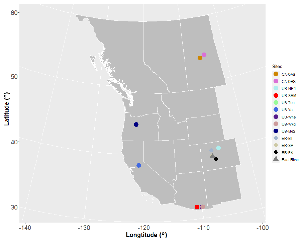
Figure 1. Location of sites considered in this study. Note that US-Ton and US-Var and US-Whs and US-Wkg are close to each other. East River Watershed is located next to ER-BT. The white lines delineate Western US states and Canadian provinces. Circles represent FLUXNET sites, diamonds represent SNOTEL sites, and the triangle represents the East River Watershed.
