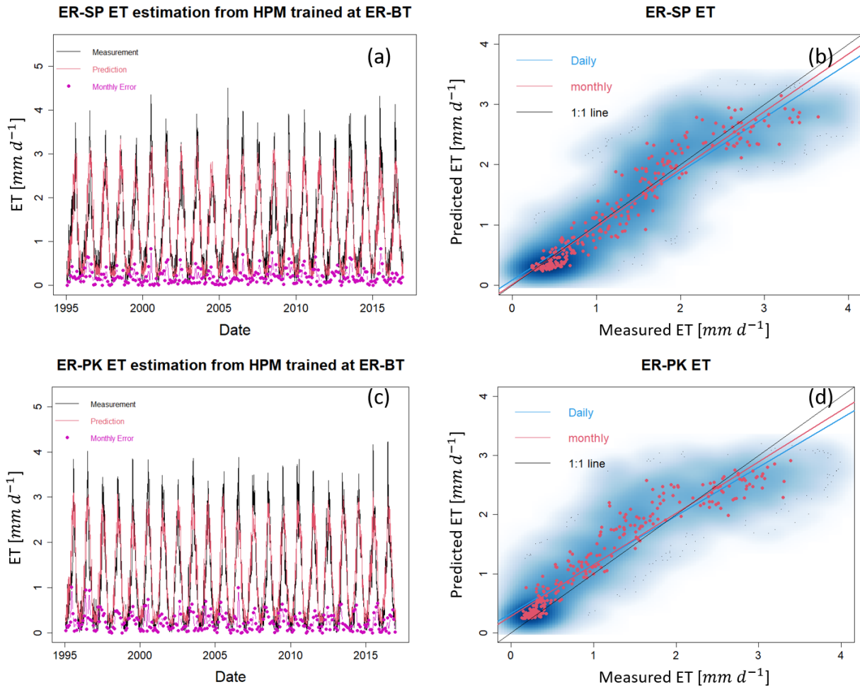
Figure 7. The HPM approach trained with CLM simulation at ER-BT is used to estimate ET at ER-SP and ER-PK. Panels (a) and (c) display the time series of HPM estimation of ET (red lines) and independent CLM estimation at ER-SP and ER-PK. Panels (b) and (d) show the scatter plots of daily (blue) and monthly (red) ET at these sites. Darker blue clouds represent greater density of data points.
