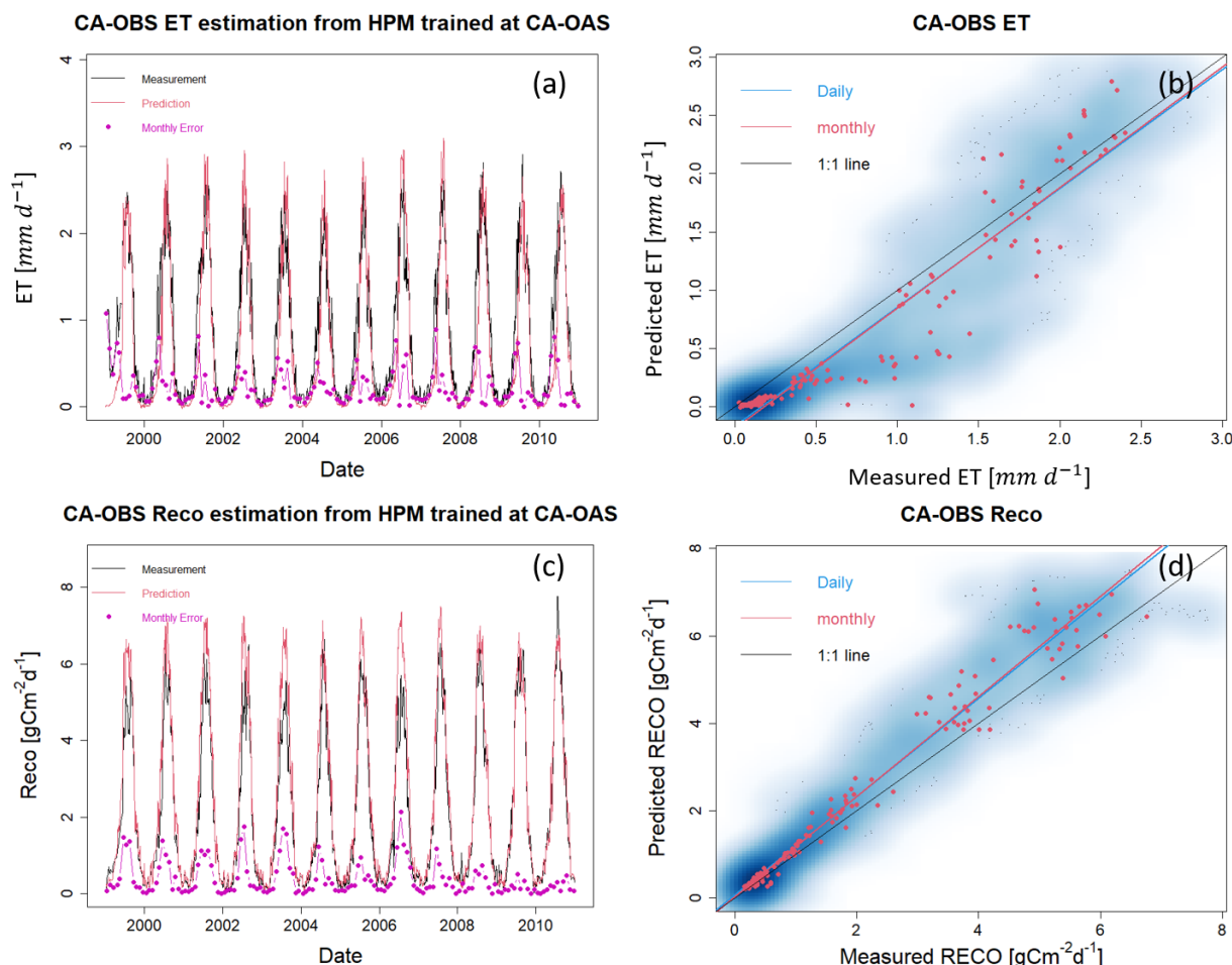
Figure 6. ET and R_{\text{eco}} estimation at CA-Obs using HPM trained at CA-Oas. Other sites are presented in Fig. A5.
