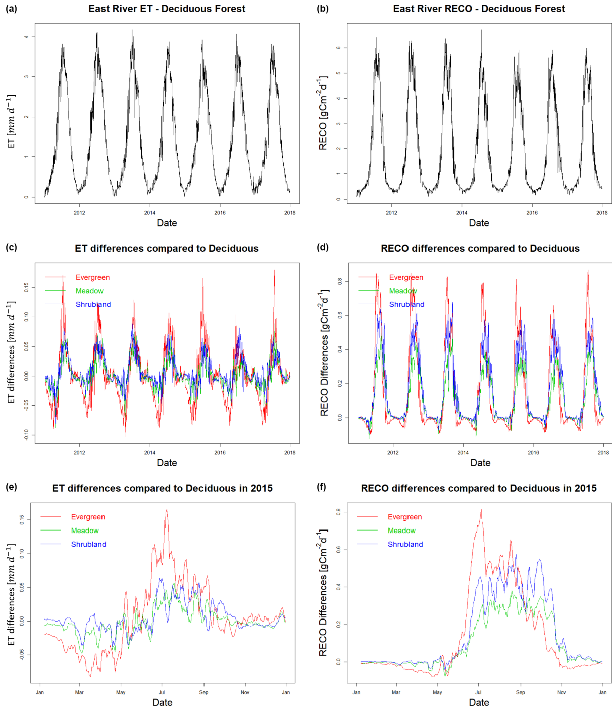
Figure 9. ET (a) and R_{eco} (b) estimation for the deciduous forest site DFI at the East River Watershed. Panels (c) and (d) show the differences in ET and R_{eco} among various vegetation types and deciduous forest. Red, green, and blue lines represent the differences in evergreen forest, meadow, and riparian shrubland compared to deciduous forest. Panels (e) and (f) zoom into 2015 to better display seasonal variations.
