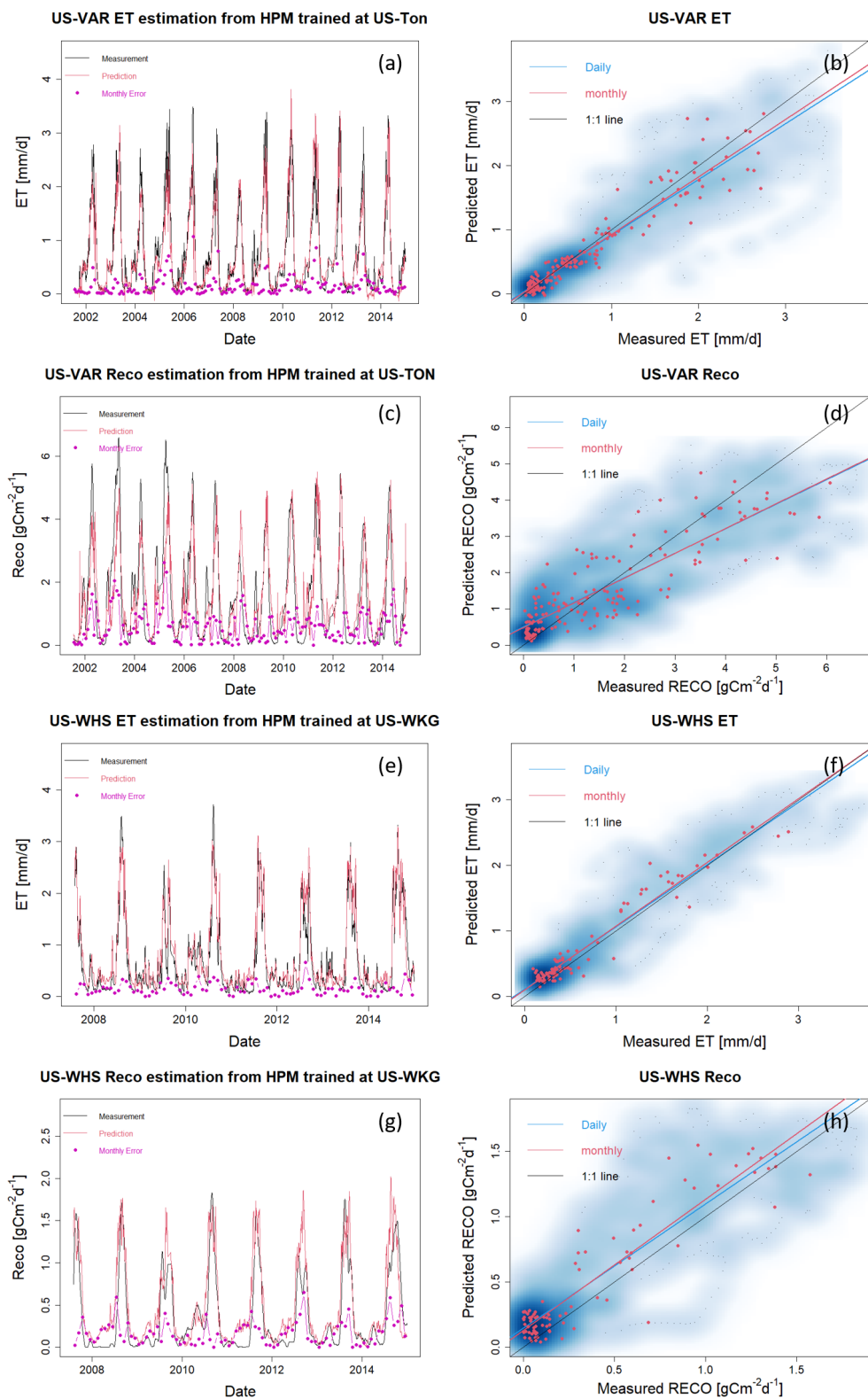
Figure A5. Use case 2. ET and R_{eco} estimation at US-Var and US-Whs from HPM trained at US-Ton and US-Wkg, respectively.
