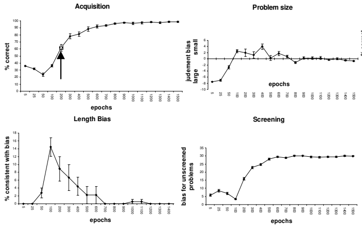
Figure 3: Developmental phases of the normal model. The arrow shows shift from NC=>C for the acquisition metric
