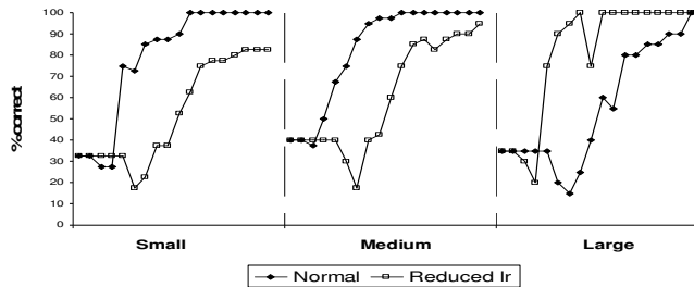
Figure 11: Profile of performance across problem types during learning for reduced lr and normal cases
