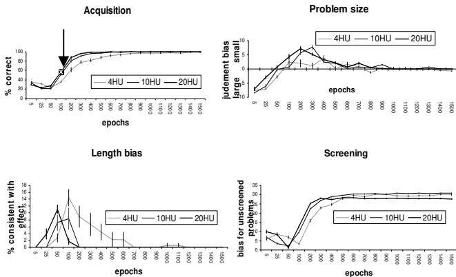
Figure 5: Profile for models with 4 (normal), 10 and 20 HU in a single layer. Arrow shows shift from NC=>C
