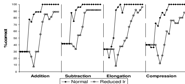
Figure 10: Profile of performance across problem types during learning for reduced lr and normal cases
