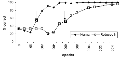
Figure 8: Training performance for the normal and reduced learning rate models. Arrows show the shift from NC=>C
