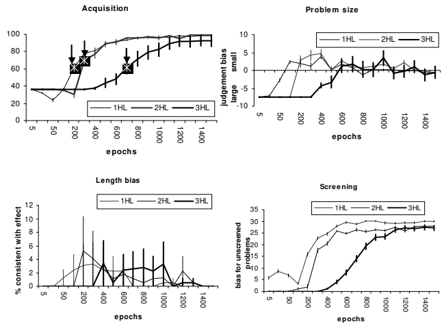
Figure 4: Profile for models with 1 (normal), 2 and 3 HL. Arrows show shifts from NC=>C
