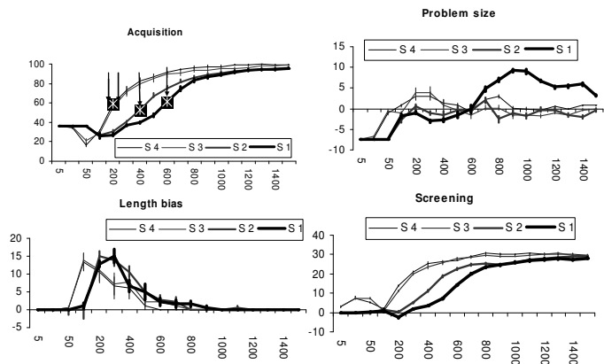
Figure 7: The 1HL model with declining sigmoid slope
