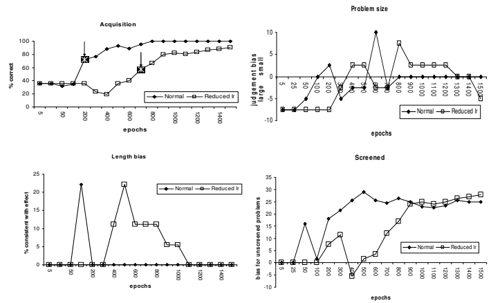
Figure 9: Profile for the normal and reduced learning rate models. Arrows show the shift from NC=>C
