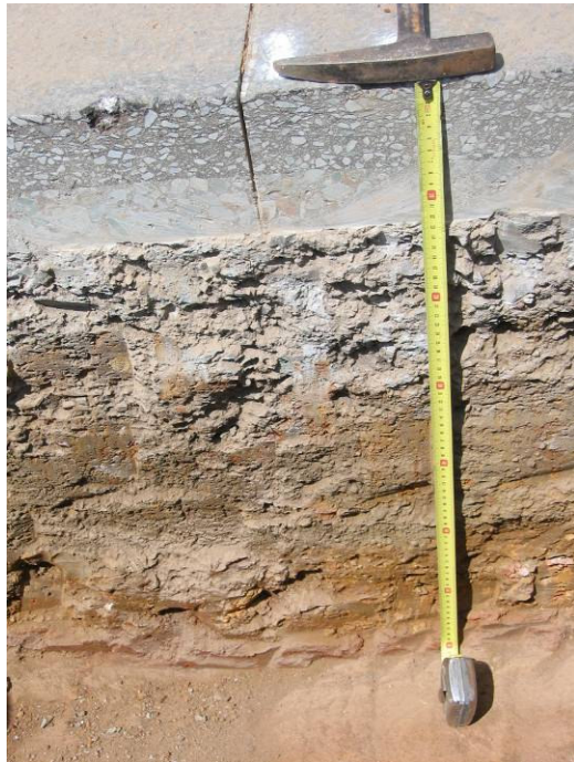
Hand-finished test pit face
