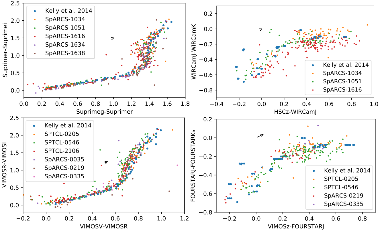
Figure A1. Different representations of the stellar locus that was used for calibration of the multi-band photometry. Thicker blue symbols : stellar spectral library from Kelly et al. (2014), convolved with the response function for different combinations of telescope optics/filter/detector/atmosphere. Top panels : filters used for some of the Northern clusters. Bottom panels : same for the Southern clusters. Left panels : Stellar locus in optical/visible filters. Right panels : Stellar locus in Near-IR. Different colours show calibrated photometry for the different clusters, after correcting for (the small amount of) galactic dust absorption (Schlegel et al. 1998). Arrows show the maximum dust extinction that was corrected for within the cluster sample.
