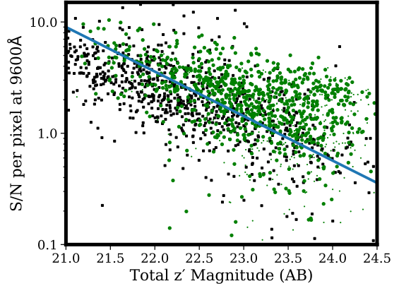
Figure 3. The S/N per 3.9\text{\AA} pixel, measured at a wavelength of 9600\text{\AA} , is shown as a function of total z' -band magnitude, for all GCLASS spectra (black squares) and GOGREEN (green dots) primary targets. Heavier symbols correspond to spectra that yield a reliable redshift (see § 4.2.1). The straight line is shown as a reference; it represents the dependence of S/N on magnitude that would be expected if all spectra were obtained in the same conditions and with the same exposure time (arbitrary normalization). This demonstrates how the longer exposure times on the faintest galaxies in GOGREEN successfully ensures that most spectra obtain S/N > 1 per pixel, independent of magnitude.
