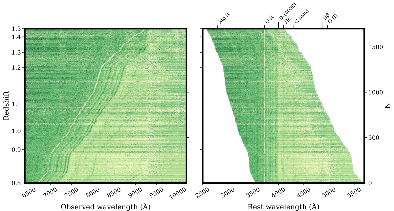
Figure 8. These figures show all GOGREEN and GCLASS spectra with robust redshifts between 0.8 < z < 1.5 . The spectra are arranged in order of increasing redshift, from bottom to top as shown on the y-axis. The left panel shows the spectra in observed wavelength, while on the right they are in rest-frame coordinates. The [O II] emission line, 4000Å break and several absorption lines (indicated at the top of the right panel) are clearly visible.
