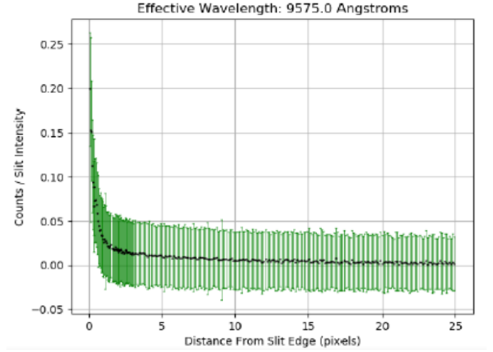
Figure B2. The average number of counts per 0.081 \text{ \AA} pixel, relative to the average slit intensity, as a function of distance away from the edge of a slit. This is shown at fixed wavelength, of 9575 \text{ \AA} . The green vertical bars show the variance among the measured slits; they are not the error on the mean, and they are not independent.
