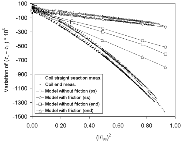
Fig. 11. Variation of bidirectional strain in the coil end regions during magnet excitation as a function of the fraction of Lorentz force with respect to the 4.5 K short sample value: \epsilon_{\perp} and \epsilon_{\parallel} are respectively the strains perpendicular and parallel to the wide surface of the cable.
