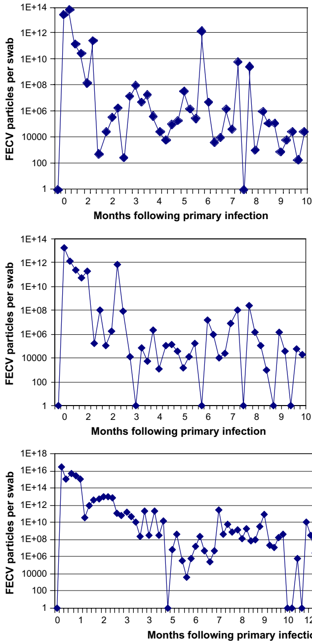
Fig 1. Typical fecal FECV shedding patterns of cats demonstrating a persistent pattern of infection.
