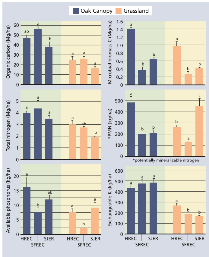
Fig. 2. Organic carbon and nutrient pools (mean \pm standard error; n = 5) for the 0-6-inch (0-15 cm) depth increment of soils beneath the oak canopy and adjacent grasslands for sites at HREC (sandstone/shale), SFREC (greenstone) and SJER (granite). Means with same lower case letters within each vegetation type (oak versus grassland) are not statistically different at P = 0.05 .
