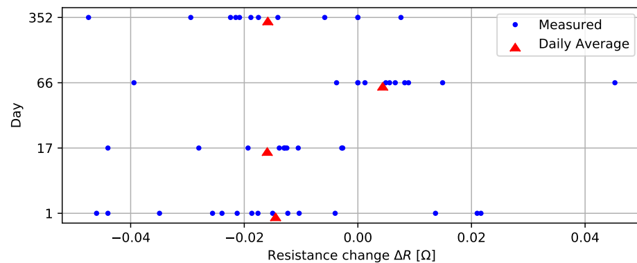
Figure 12. Trace resistance over time.
