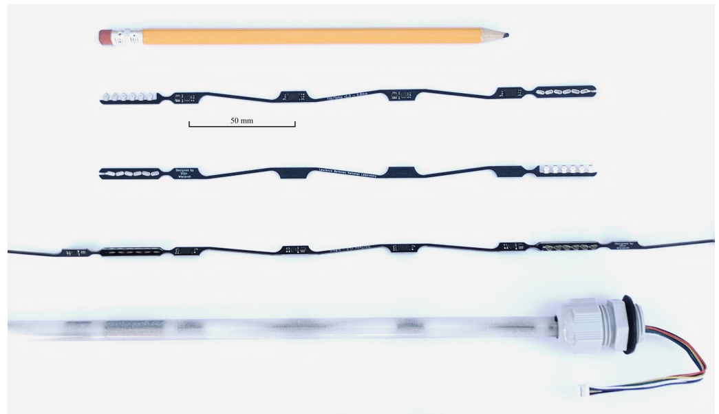
Figure 4. Modular design of the sensor probe. From top to bottom: top view of a sensor board, bottom view of a sensor board, cascaded sensor boards, and final probe assembly containing an array of cascaded sensor sections in a 3/8 in. (~10 mm) outer diameter tube, filled with epoxy.
