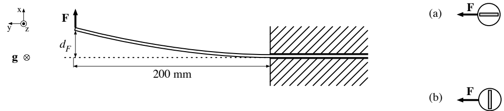
Figure 5. Test setup to measure the deformation d_F of a 20 cm long probe segment as a result of a sideways force F , which is applied (a) in the PCB plane, or (b) perpendicular to the PCB plane.
