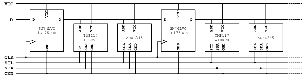
Figure 2. Schematic of cascaded temperature sensors and accelerometers in a shift register configuration
