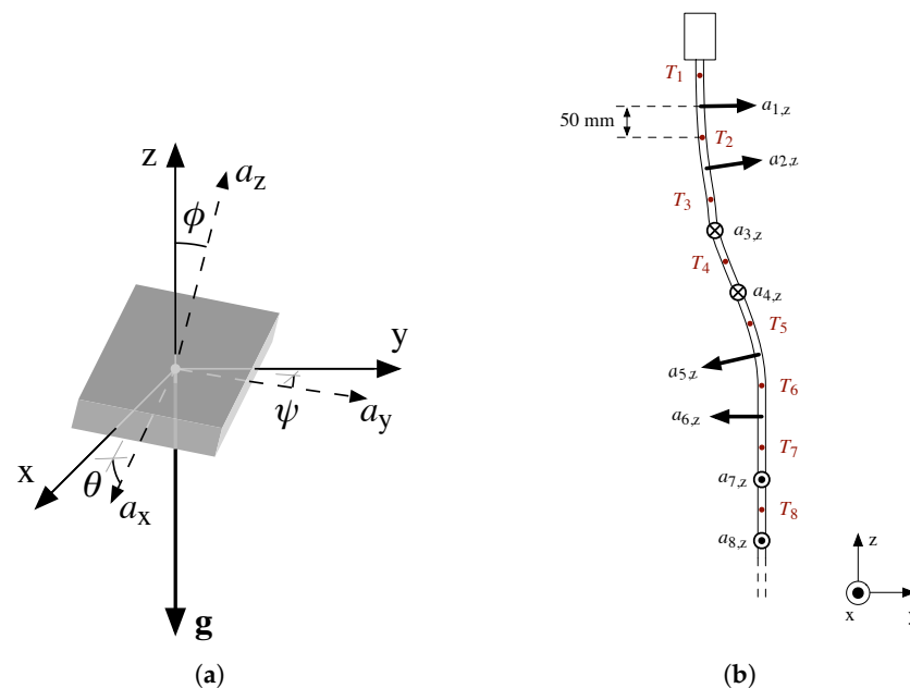
Figure 1. Accelerometer arrays can be used for deformation measurements. (a) Inclinometer measurement with an accelerometer and (b) design of the probe with temperature sensors ( T_i ) and accelerometers ( a_i ).
