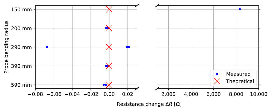
Figure 11. Trace resistance under bending.
