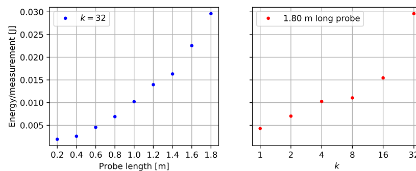
Figure 7. Energy per measurement as a function of probe length or the number of averaged measurements ( k ).
