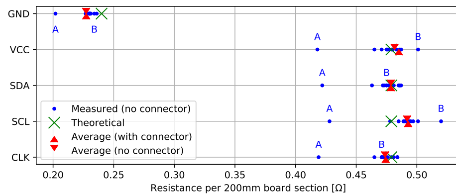
Figure 9. Trace resistance per 200 mm probe section, with and without connectors. Outlying trace resistance values for the same board are labeled as ‘A’ or ‘B’.
