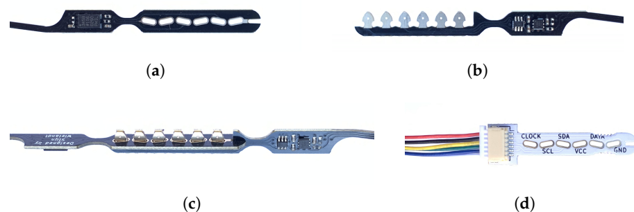
Figure 3. Close-ups of the proposed connector technology. (a) Female connector piece; (b) Male connector piece; (c) Mated connector; (d) Wire-to-Board adapter.
