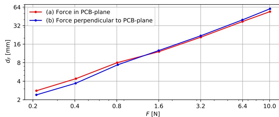
Figure 8. Deformation d_F of a 200 mm long probe segment as a result of a sideways force F , either (a) in the PCB plane or (b) perpendicular to the PCB plane.
