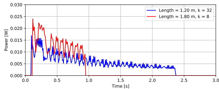
Figure 6. Power profiles for a 1.20 m long probe with 32 averaged measurements and a 1.80 m long probe with 8 averaged measurements.
