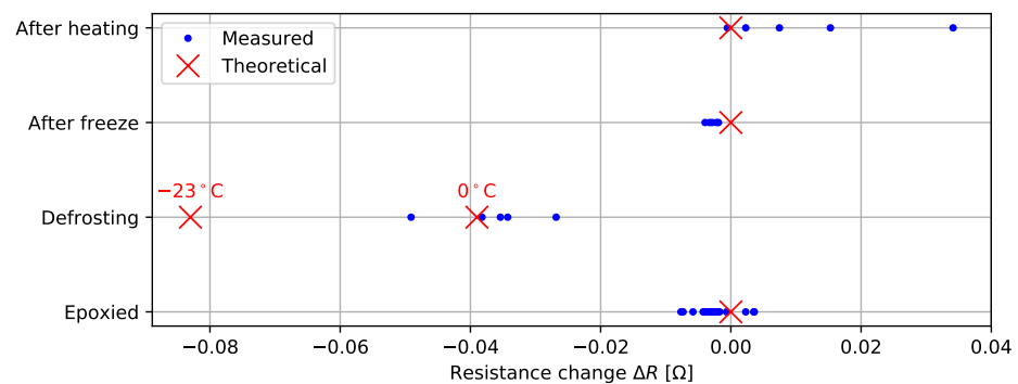
Figure 10. Trace resistance under freezing, heating, and epoxying.
