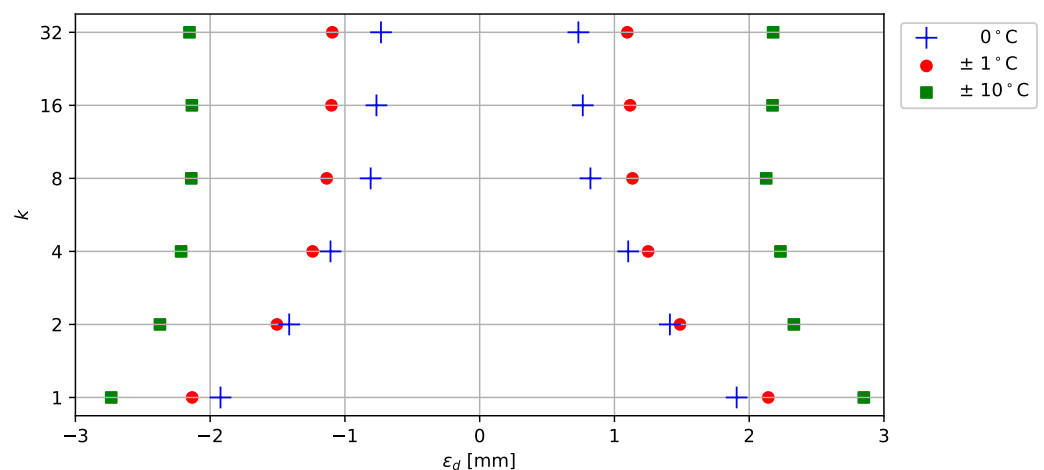
Figure 13. Deformation error ( \epsilon_d ) in function of number of averaged measurements ( k ) expressed as 2.5th and 97.5th percentiles for 0^\circ\text{C} , \pm 1^\circ\text{C} and \pm 10^\circ\text{C} temperature variations.
