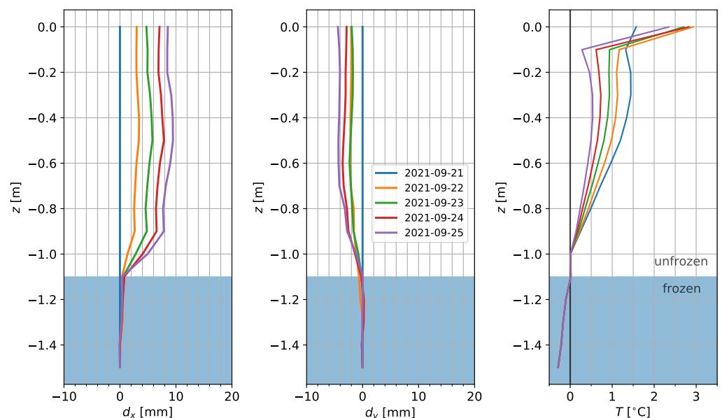
Figure 14. Field measurements obtained over five days at a field site on the Seward Peninsula, AK which is experiencing soil movements in response to permafrost thaw. Left and middle panels show the displacement along the x and y -axis, respectively; right column shows the soil temperature. Highlighted in blue is the frozen part of the subsurface, showing that the slip plane is collocated with the interface between frozen and unfrozen soil.
