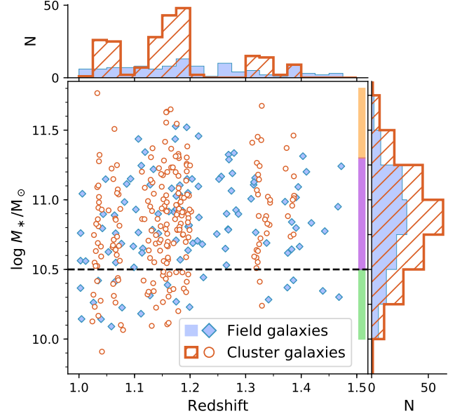
Figure 2. Stellar masses and redshifts for the UVJ -quiescent GOGREEN spectroscopic sample, with corresponding histograms on each axis. Field galaxies are shown as blue diamonds, and cluster member galaxies are red. Coloured blocks indicate the span of mass bins discussed throughout the analysis. A dashed line indicates the mass-completeness of our sample, where the lowest mass bin is below this threshold. Note that the stellar masses shown here are derived with nonparametric SFHs, and are systematically offset from those derived using FAST as reported in other GOGREEN papers, see Section 3 and Appendix C for details. Our sample ranges between 1 < z < 1.5 , and stellar masses between 10^{9.9} M_{\odot} and 10^{11.8} M_{\odot} .
