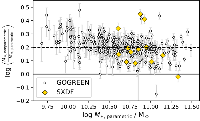
Figure C1. Comparison of FAST (parametric) and PROSPECTOR (nonparametric) derived stellar masses. We confirm the systematic offset reported by Leja et al. (2019b) that nonparametric SFHs yield larger masses, by \sim 0.2 dex (shown as a dashed line), with a mild mass dependence. Yellow diamonds indicate SXDF galaxies which have parametric stellar masses from Mehta et al. (2018) .
