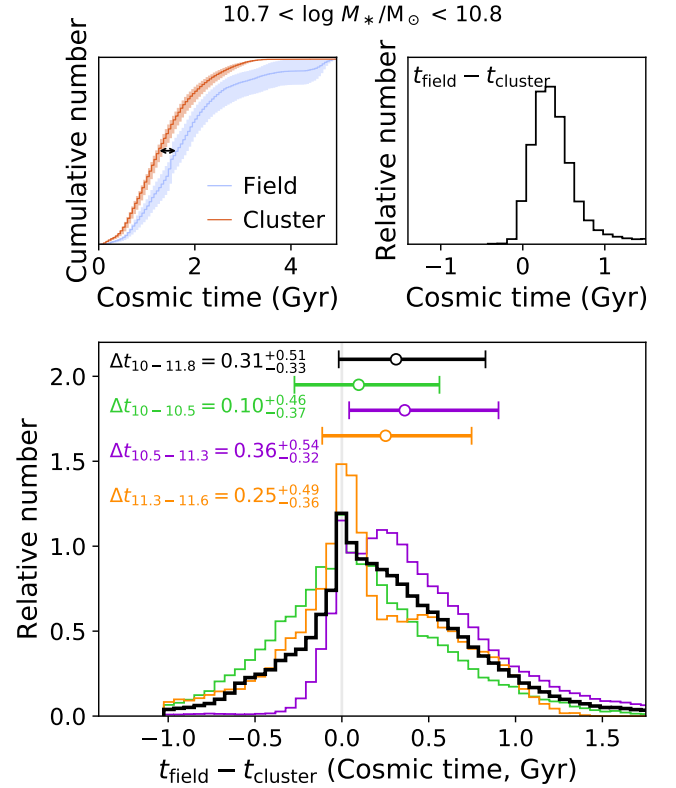
Figure 7. Distributions of offsets between cumulative age distributions of field and cluster galaxies (shown in Figure 6 as non-cumulative histograms), in units of cosmic time. The top row shows an example of this age comparison for galaxies with stellar masses 10.7 < \log M_*/M_{\odot} < 10.8 . The cumulative mass-weighted age distributions for the field (blue) and cluster (red) galaxies is shown on the top left, where the samples have been bootstrapped and the variance is shown as a shaded region. The solid lines show the medians of the bootstrapped distributions. The corresponding offsets in the mass-weighted ages for interpolated bins spanning the cumulative distributions are shown in the top right plot. Galaxies are compared at fixed stellar mass (bins of 0.1 dex) and combined, weighted by the integrated mass within the bins. The combined distributions within the broader mass selections used throughout previous figures are included for reference: 10 < \log M_*/M_{\odot} < 10.5 , green; 10.5 < \log M_*/M_{\odot} < 11.3 , purple; 11.3 < \log M_*/M_{\odot} < 11.8 , orange. The full mass range combined distribution is shown in black. The median age difference for each mass selection is labelled in the figure, which shows the age difference is within 0.31^{+0.51}_{-0.33} Gyr. The median age difference is larger at lower stellar masses, and smaller for the highest mass galaxies. Error bars indicate the 68 per cent confidence range. This quantitative comparison echoes the qualitative comparison shown in Figure 6 in that the quiescent cluster galaxies are on average older than comparable field galaxies.
