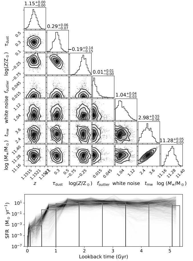
Figure 4. Selected posteriors for the fitting result shown in Figure 3, which is a typical galaxy from our sample of GOGREEN quiescent galaxies. Top: corner plot showing a selection of posterior distributions for SFH parameters: redshift, metallicity, dust opacity, outlier fraction, and white noise, as well as two derived parameters: mass-weighted age and stellar mass (see Section 3). Posteriors are shown smoothed with a 1\sigma Gaussian, and the 50 th percentiles are indicated on the top of each histogram with 68 per cent credible regions. Bottom: The posteriors for the SFRs are shown as a function of lookback time, where age bins are drawn with heights equal to the median in each bin.
