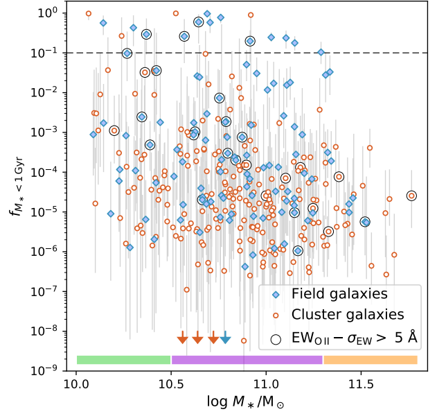
Figure 9. The fraction of stellar mass formed within the last 1 Gyr as a function of total stellar mass, for our UVJ -selected sample of quiescent galaxies. Galaxies with \text{EW}([\text{O II}]) - \sigma_{\text{EW}} > 5 \text{ \AA} are circled. Field galaxies are shown as blue diamonds, and cluster galaxies as orange circles. Arrows indicate points below the shown scale. ‘Young’ f_{M_*, < 1 \text{ Gyr}} > 0.1 galaxies are more common among field galaxies, and at stellar masses < 10^{11.3} M_{\odot} . There is no correlation between the presence of [O II] emission and f_{M_*, < 1 \text{ Gyr}} > 0.1 , however. The robustness of age-comparison is tested by excluding this population of ‘young’ galaxies, see Figure 8.
