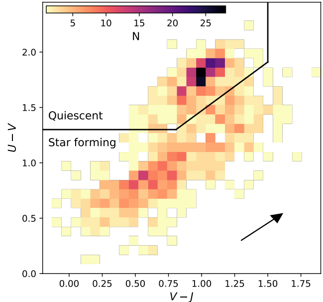
Figure 1. Rest-frame UVJ colours for the GOGREEN spectroscopic sample between 1 < z < 1.5 , shown as a 2D histogram for both cluster and field galaxies. The black line shows the selection of quiescent galaxies used in this study, as defined by Muzzin et al. (2013b), from star forming galaxies. The arrow indicates the impact of 1 mag of extinction in the V -band, using the Calzetti et al. (2000) dust law.
