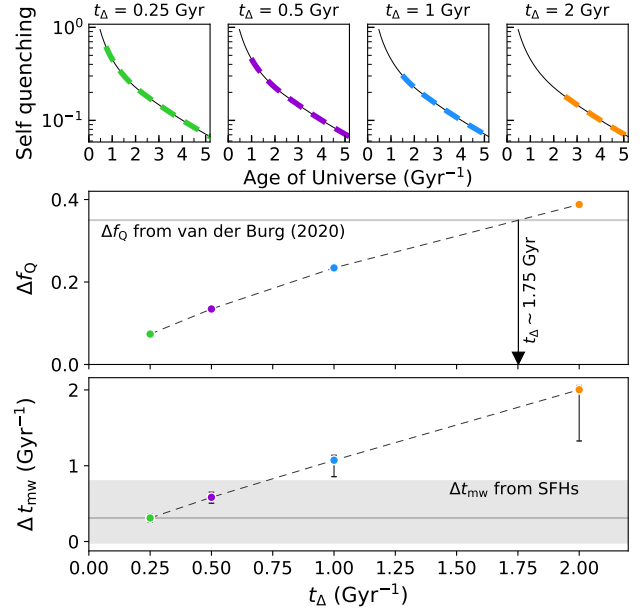
Figure 11. Toy model of the expected difference in quenched fractions and t_{\text{mw}} given an offset in the formation of the field population of t_{\Delta} . Top: quenching rate for four values of t_{\Delta} : 0.25 Gyr, 0.5 Gyr, 1 Gyr, and 2 Gyr. The cluster quenching rate is shown as a black line starting at z_{\text{form}}=10 , and field quenching rate as a coloured (according to t_{\Delta} ) dashed line. Middle: The difference in quenched fractions, \Delta f_Q , for fixed stellar mass at z=1.2 , for the four t_{\Delta} models shown. Larger offsets in the formation of field galaxies corresponds to larger \Delta f_Q . A horizontal line indicates the measured difference in quenched fractions from van der Burg et al. (2020). Bottom: Average difference in cumulative t_{\text{mw}} distributions, \Delta t_{\text{mw}} , between field and cluster galaxies, with error bars indicating the 68 per cent spread. The grey shaded region indicates the measured average age difference, see Section 4.2. Larger offsets in the formation of field galaxies corresponds to larger \Delta t_{\text{mw}} . In the context of this simple model, t_{\Delta} < 0.75 Gyr is consistent with our observations, but is inconsistent with the time derived by the difference in quenched fractions.
