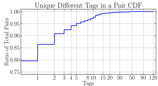
Figure 1: Overview of website pairs that have at most x tags unmatched tags (removed and inserted tags are combined).
