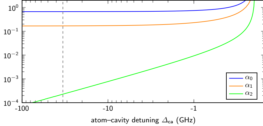
Figure 3.1: Coupling coefficients describing the interaction given by Eqn. 3.5. At \Delta_{\text{ca}}/2\pi = -33.5 GHz (experimental value, gray dashed line), the tensor coupling \alpha_2 is negligible, and the scalar and vector coupling coefficients have reached their asymptotic values.
