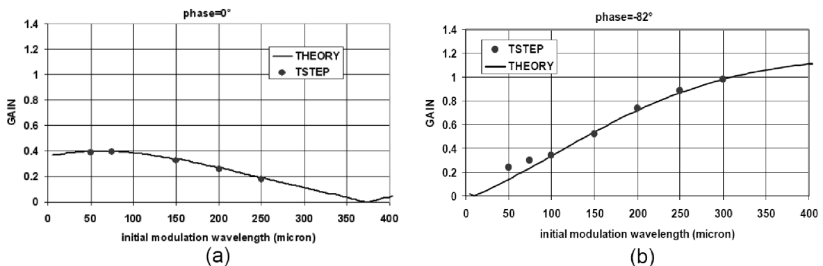
FIG. 11: Comparison between TSTEP simulations and linear theory for the linear gain through the bunch compressor over a spectrum of perturbation wavelengths; (a) is for a beam accelerated ‘on crest’ (uncompressed) C=1 , (b) for compression factor C=2 .
