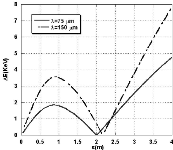
FIG. 5: Amplitude of the energy modulation amplitude along the rf compressor resulting from an initial density modulation with 10% amplitude relative to an initial current I_0 = 100A . Other beam and rf compressor parameters as in Fig. ?? and ??.
