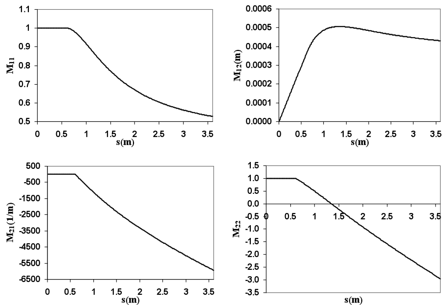
FIG. 2: Entries of the transfer matrix M for k_{rf}=59.8 \text{ m}^{-1} , \alpha=0.82 , \psi_0=-8^\circ , \gamma_{r0}=12 .
