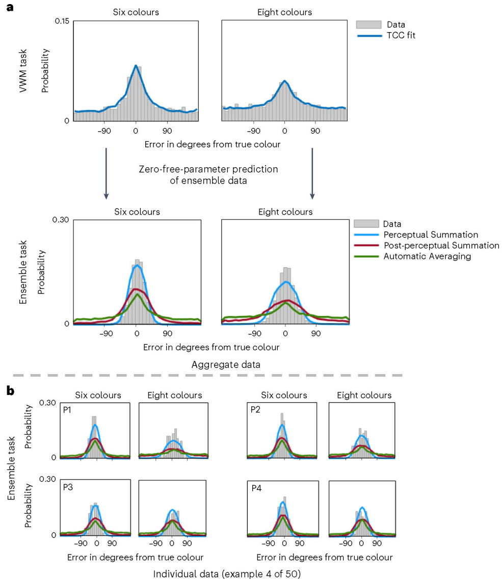
Fig. 7 |. The Perceptual Summation model predicts ensemble memory for colour with set size manipulation.
