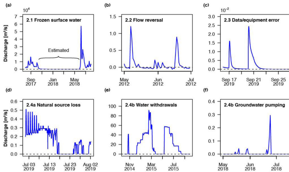
Figure 3. Examples of daily hydrographs displaying zero-flow readings. (a) Kuparuk River, near Deadhorse, AK (USGS site: 15896000), (b) Berger Ditch near Oregon, OH (USGS site: 04194085), (c) Rio Puerco near Bernardo, NM (USGS site: 08353000, provisional data downloaded September 26, 2019), (d) Agua Fria River Near Mayer, AZ (USGS site: 09512500, provisional data downloaded Sep. 26, 2019), (e) Snake River near Milner Dam, ID (non-USGS gage), and (f) Arkansas River at Garden City, KS (USGS site: 07139000). Subplot subtitles indicate the associated zero-flow scenarios as illustrated in Figure 2. Data source: U.S. Geological Survey, 2019
